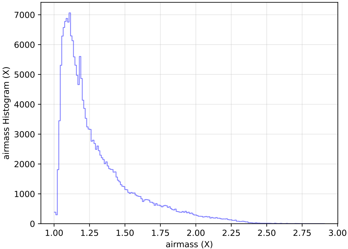
too_elab_r16_d2_ugrizy_v3.4_10yrs WFD g band: airmass Histogram
