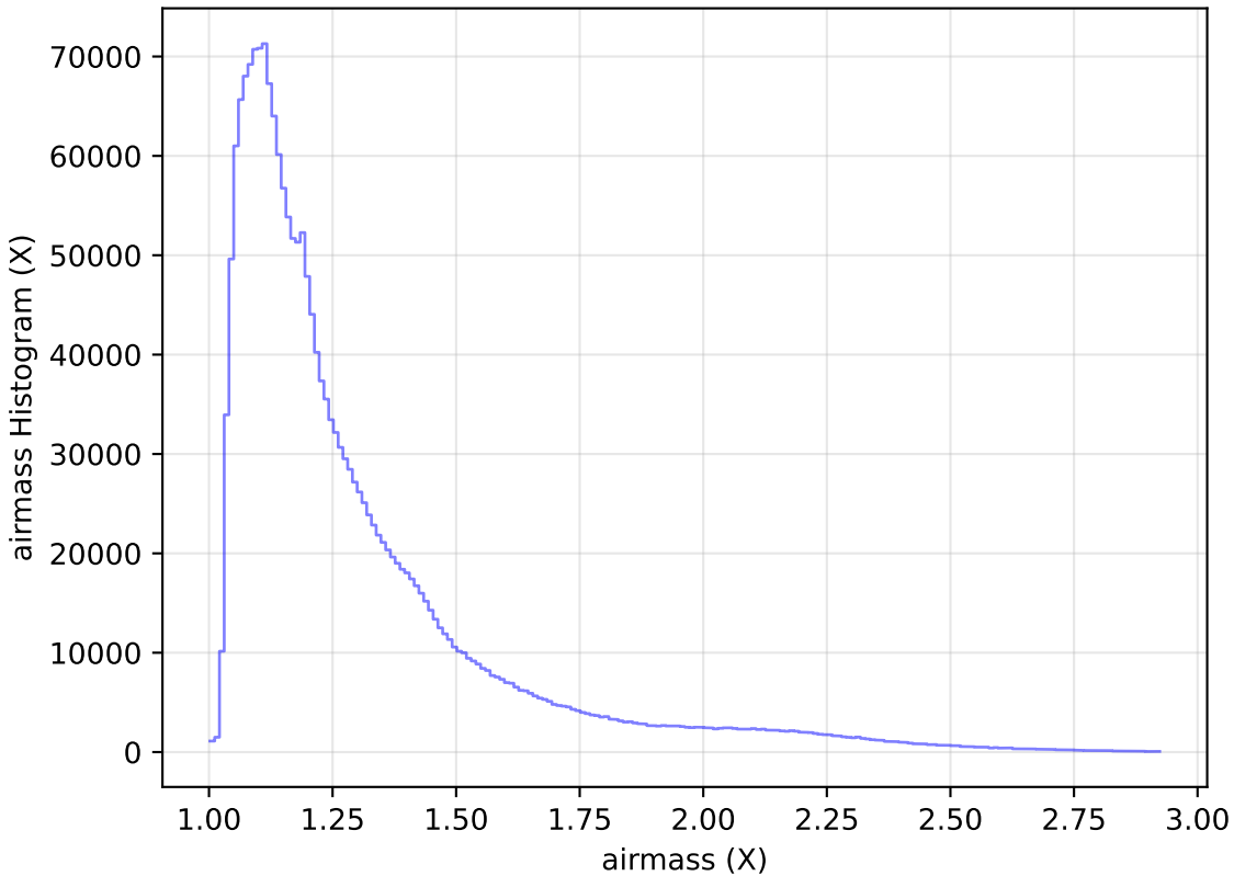
too_elab_r16_d2_ugrizy_v3.4_10yrs WFD all bands: airmass Histogram
