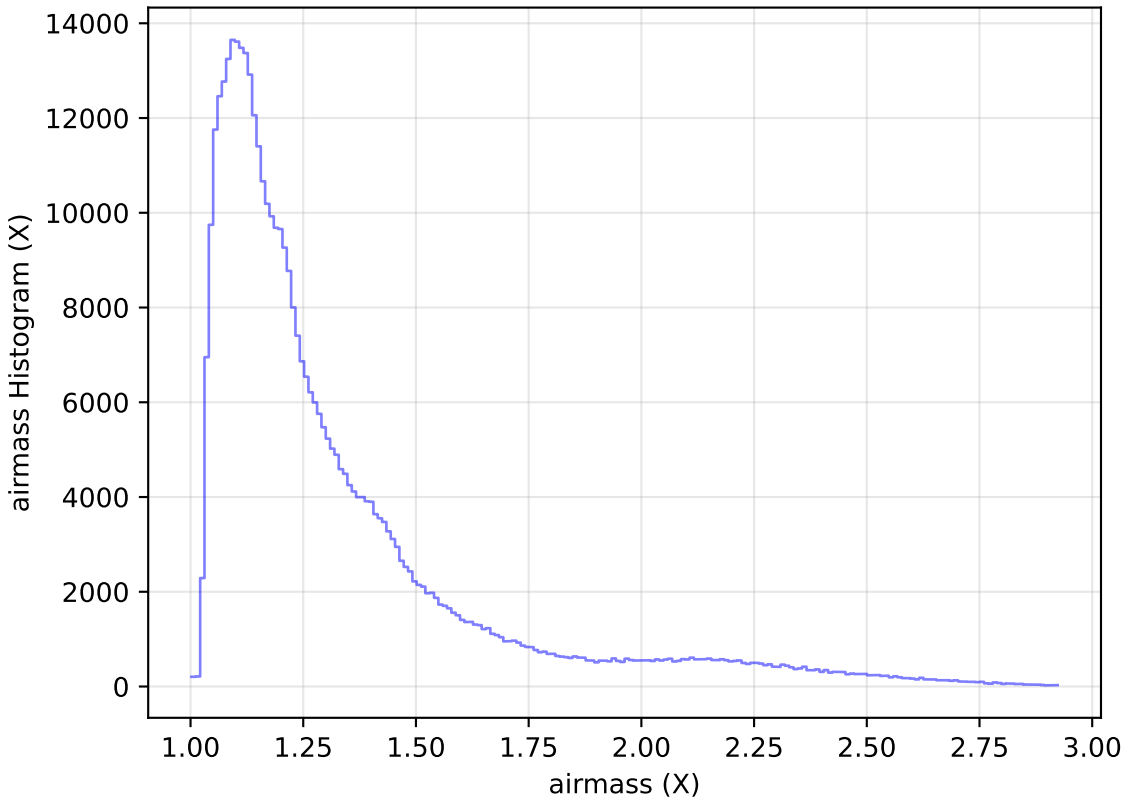
too_elab_r16_d2_ugrizy_v3.4_10yrs All sky z band: airmass Histogram
