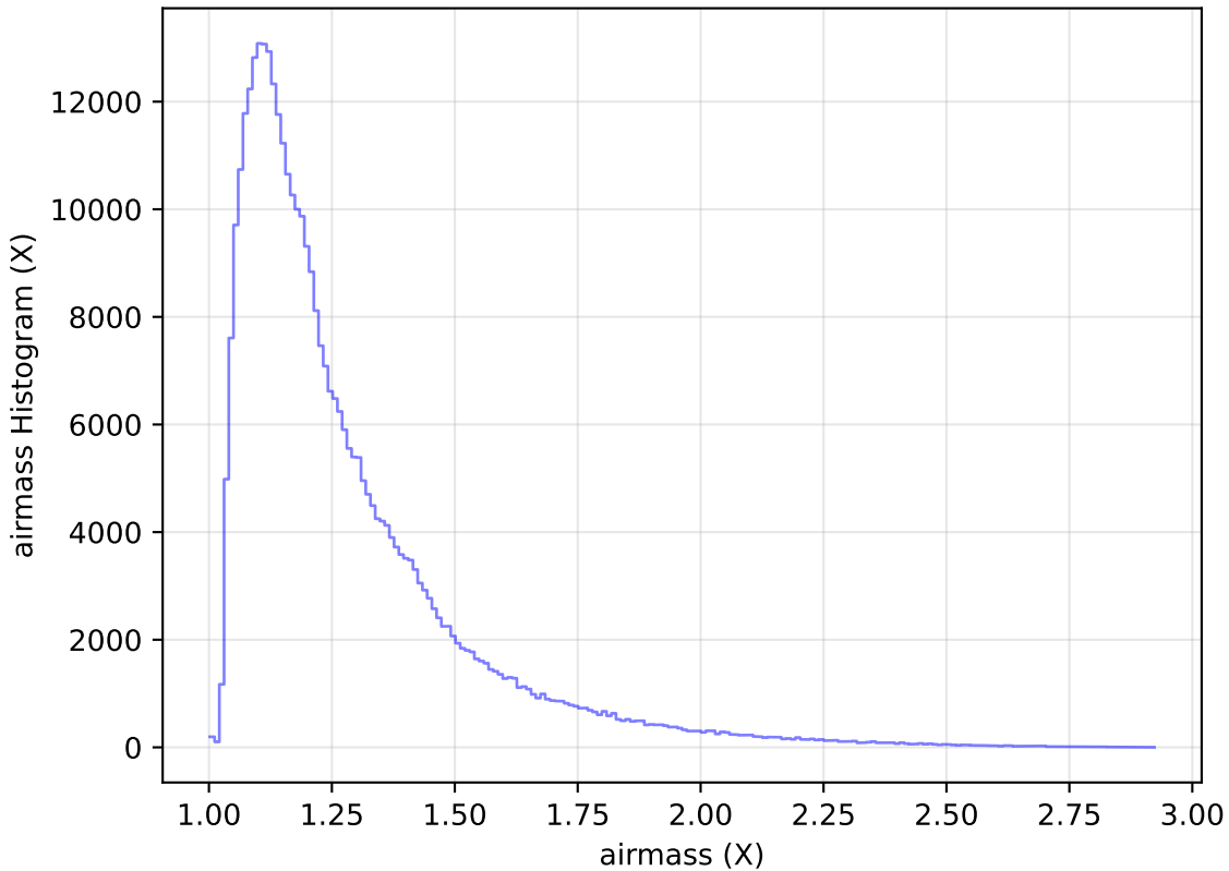
too_elab_r16_d2_ugrizy_v3.4_10yrs All sky y band: airmass Histogram
