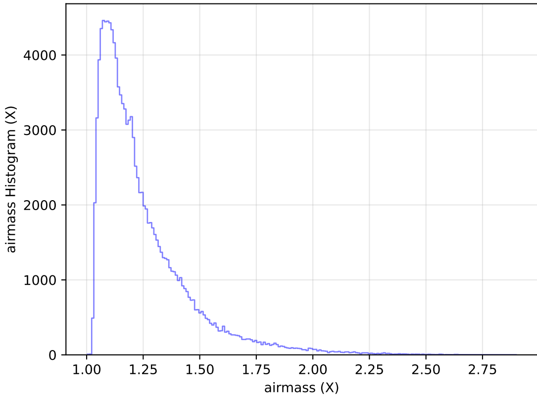
too_elab_r16_d2_ugrizy_v3.4_10yrs All sky u band: airmass Histogram
