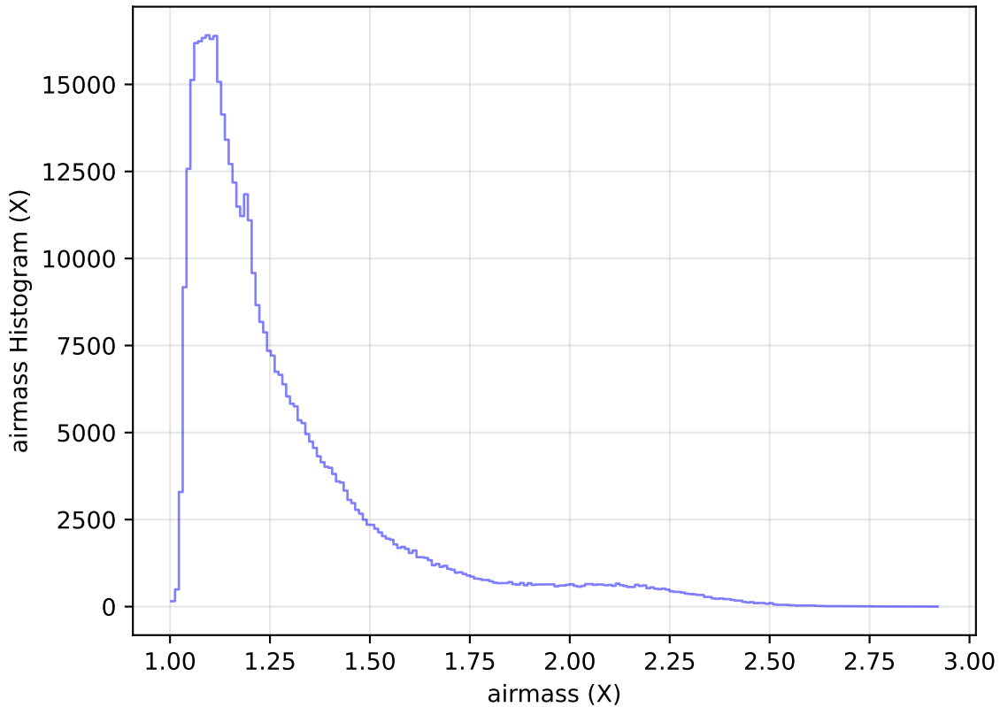
too_elab_r16_d2_ugrizy_v3.4_10yrs All sky r band: airmass Histogram
