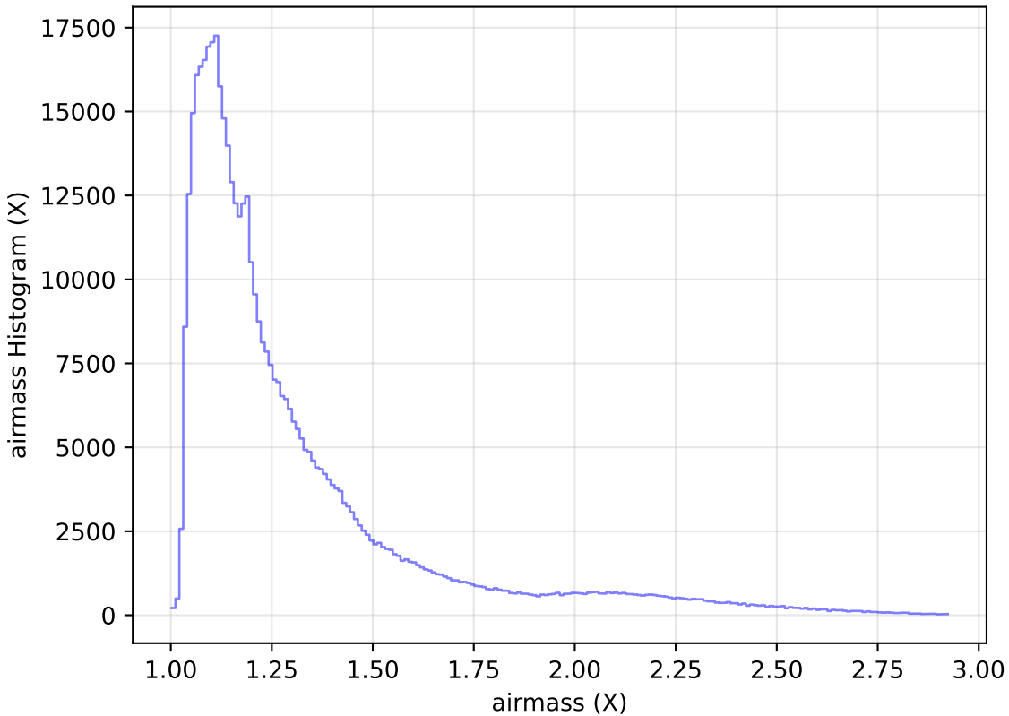
too_elab_r16_d2_ugrizy_v3.4_10yrs All sky i band: airmass Histogram
