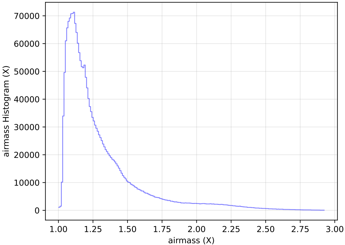
too_elab_r16_d2_ugrizy_v3.4_10yrs All sky all bands: airmass Histogram
