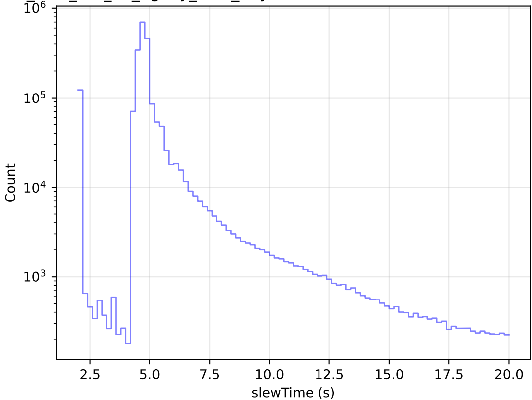
too_elab_r16_d2_ugrizy_v3.4_10yrs All visits: Zoom Slew Time Histogram
