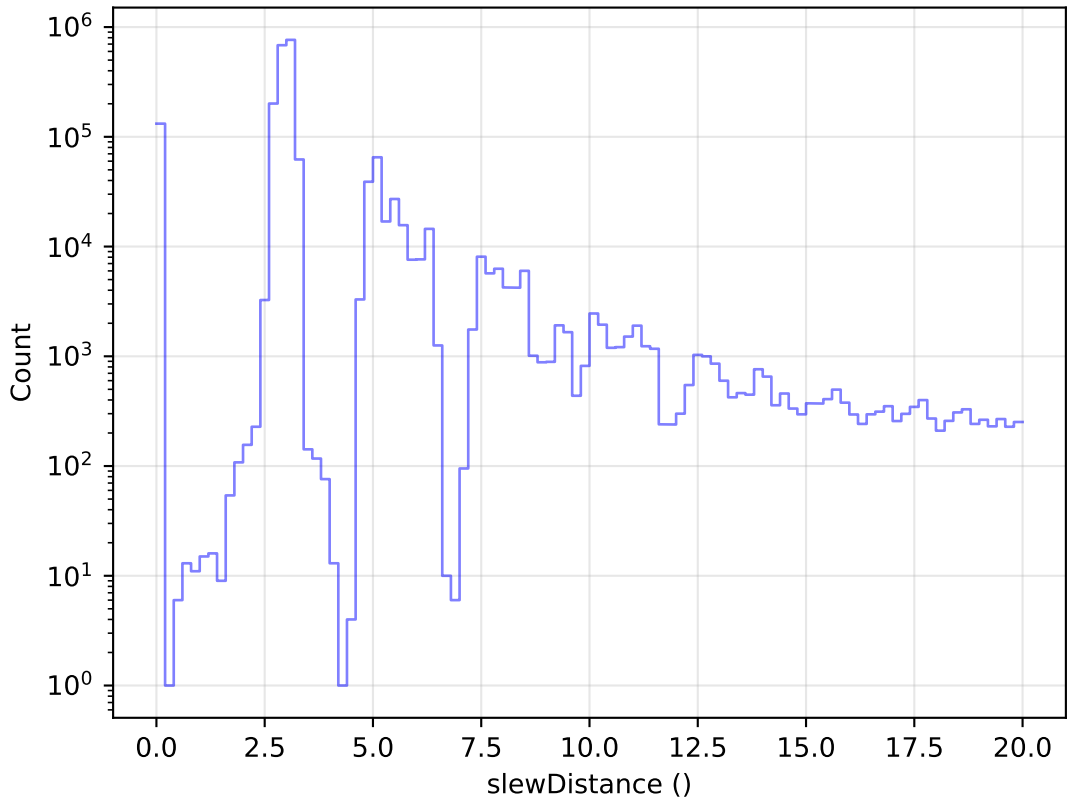
too_elab_r16_d2_ugrizy_v3.4_10yrs All visits: Zoom Slew Distance Histogram
