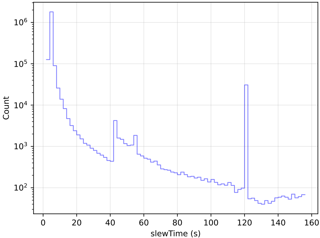
too_elab_r16_d2_ugrizy_v3.4_10yrs All visits: Slew Time Histogram
