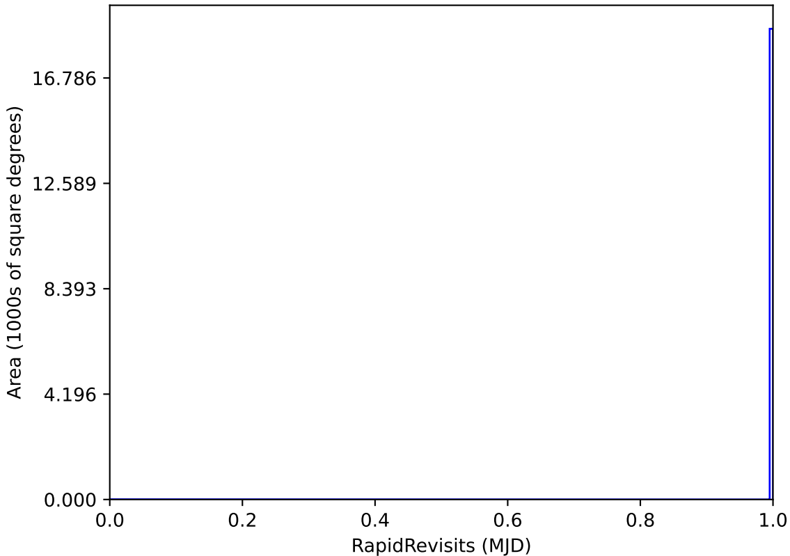
too_elab_r16_d2_ugrizy_v3.4_10yrs WFD: RapidRevisits
