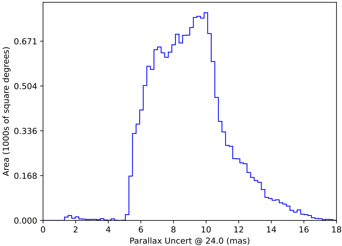
too_elab_r16_d2_ugrizy_v3.4_10yrs WFD: Parallax Uncert @ 24.0
