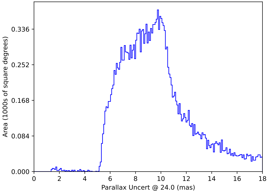
too_elab_r16_d2_ugrizy_v3.4_10yrs All sky: Parallax Uncert @ 24.0
