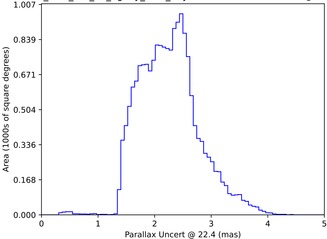
too_elab_r16_d2_ugrizy_v3.4_10yrs WFD: Parallax Uncert @ 22.4
