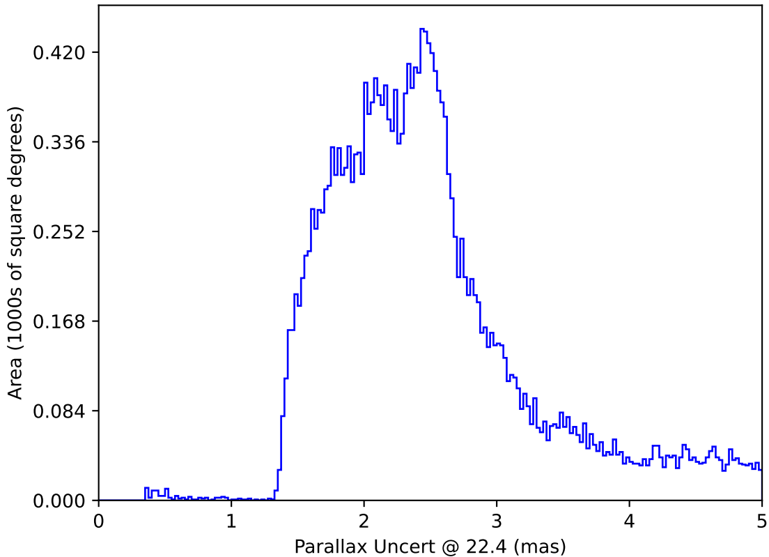
too_elab_r16_d2_ugrizy_v3.4_10yrs All sky: Parallax Uncert @ 22.4
