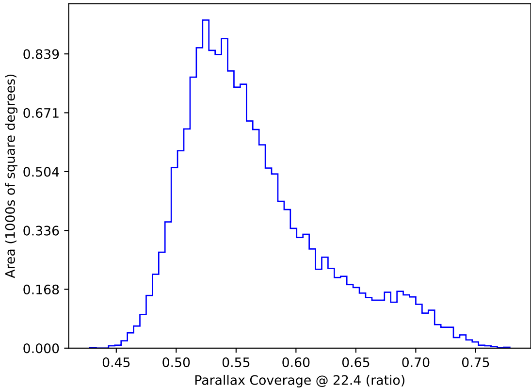
too_elab_r16_d2_ugrizy_v3.4_10yrs WFD: Parallax Coverage @ 22.4
