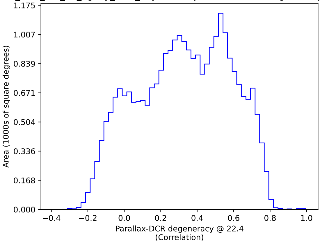
too_elab_r16_d2_ugrizy_v3.4_10yrs All sky: Parallax-DCR degeneracy @ 22.4
