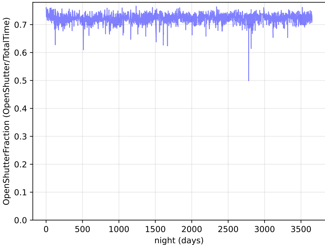
too_elab_r16_d2_ugrizy_v3.4_10yrs Per night: OpenShutterFraction
