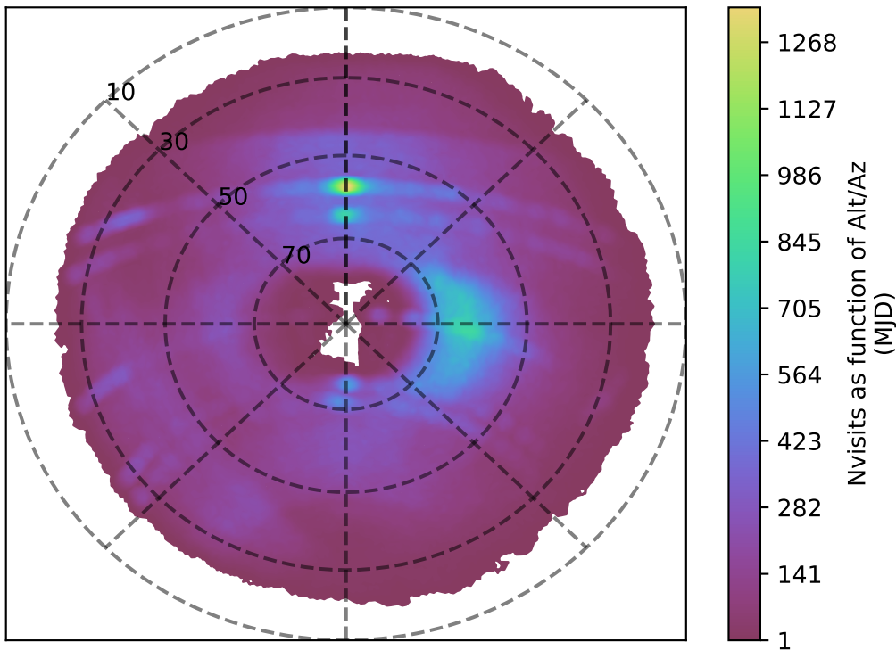
too_elab_r16_d2_ugrizy_v3.4_10yrs g band: Nvisits as function of Alt/Az
