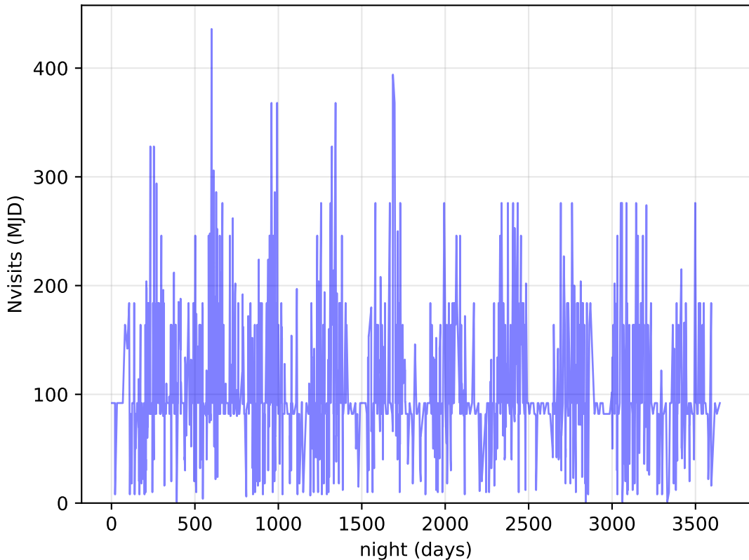
too_elab_r16_d2_ugrizy_v3.4_10yrs DDF: Nvisits
