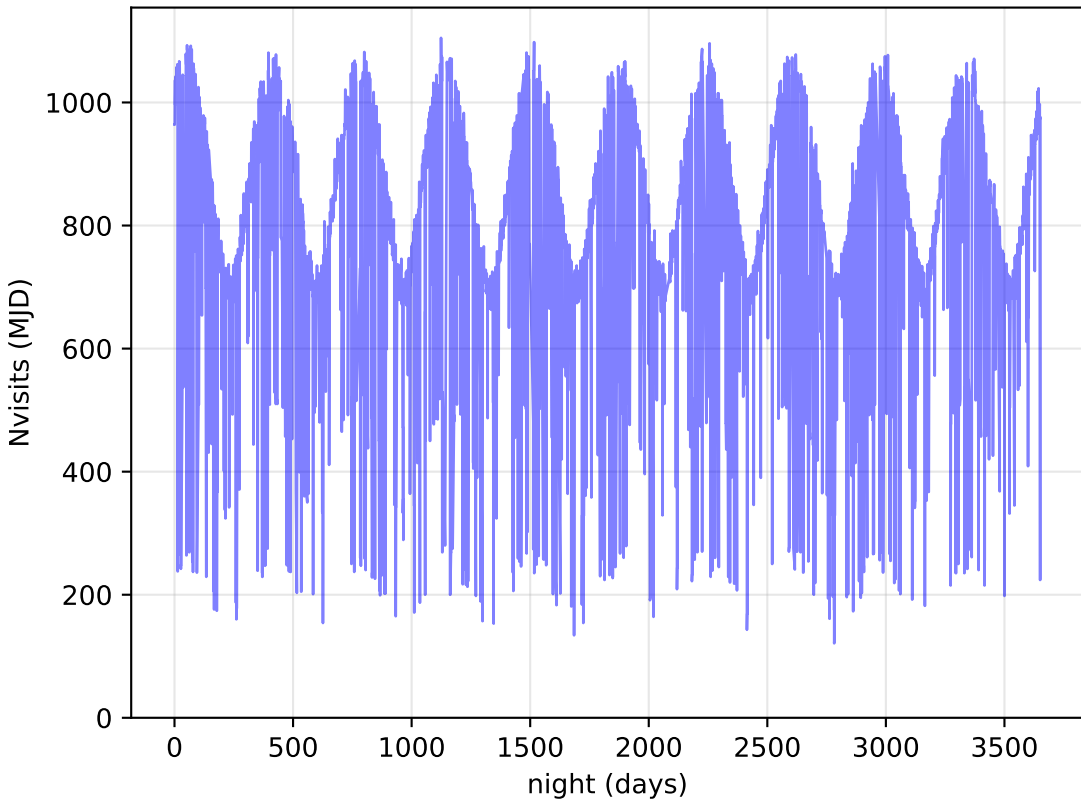
too_elab_r16_d2_ugrizy_v3.4_10yrs All visits: Nvisits
