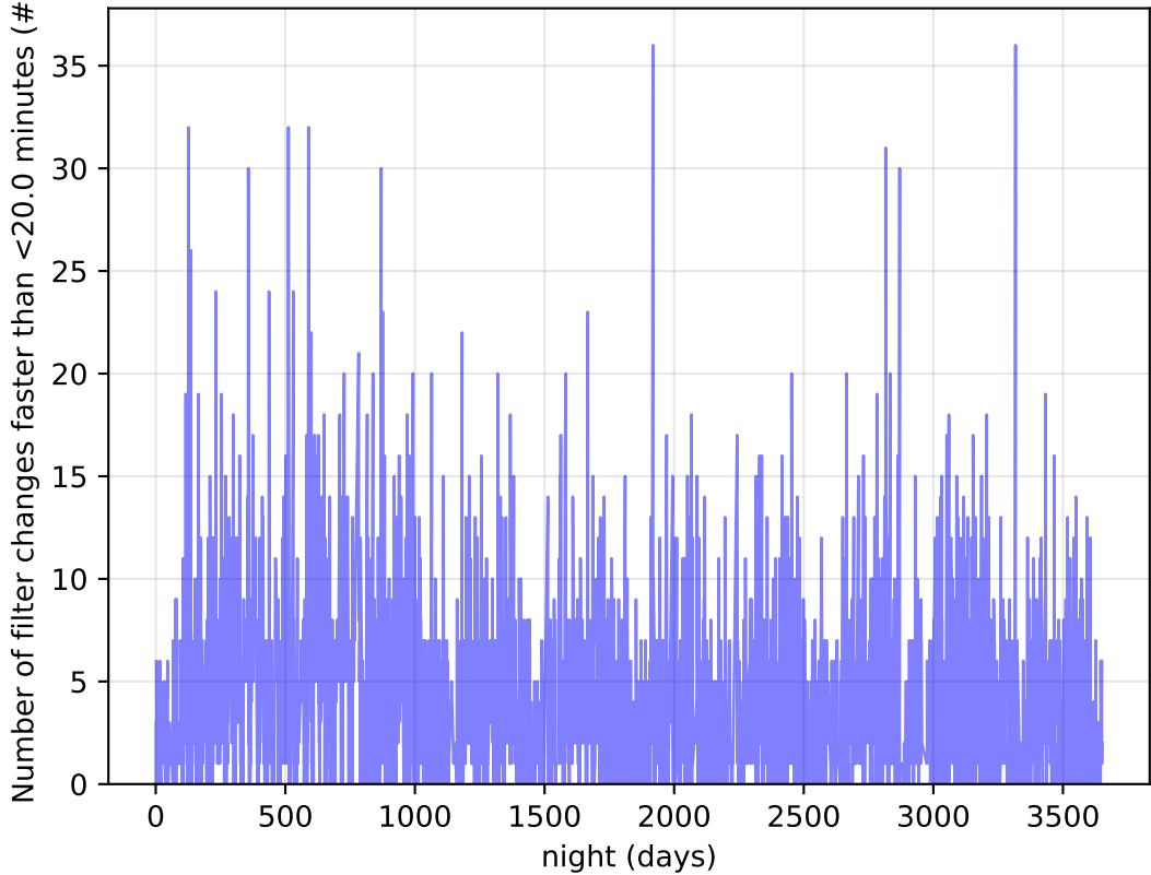
too_elab_r16_d2_ugrizy_v3.4_10yrs Per Night: Number of filter changes faster than <20.0 minutes
