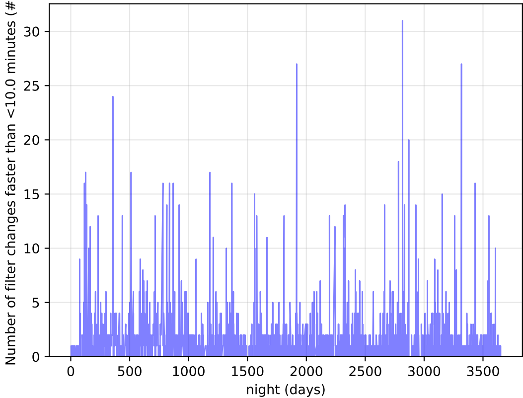
too_elab_r16_d2_ugrizy_v3.4_10yrs Per Night: Number of filter changes faster than <10.0 minutes
