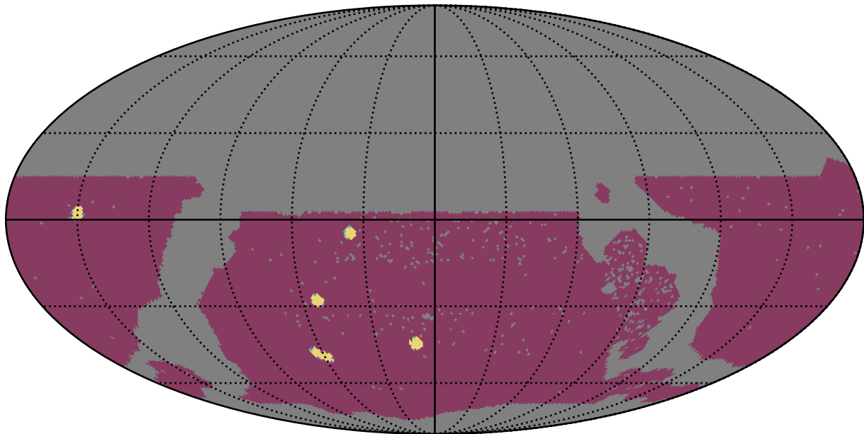
too_elab_r16_d2_ugrizy_v3.4_10yrs WFD: NumberOfQuickRevisits
