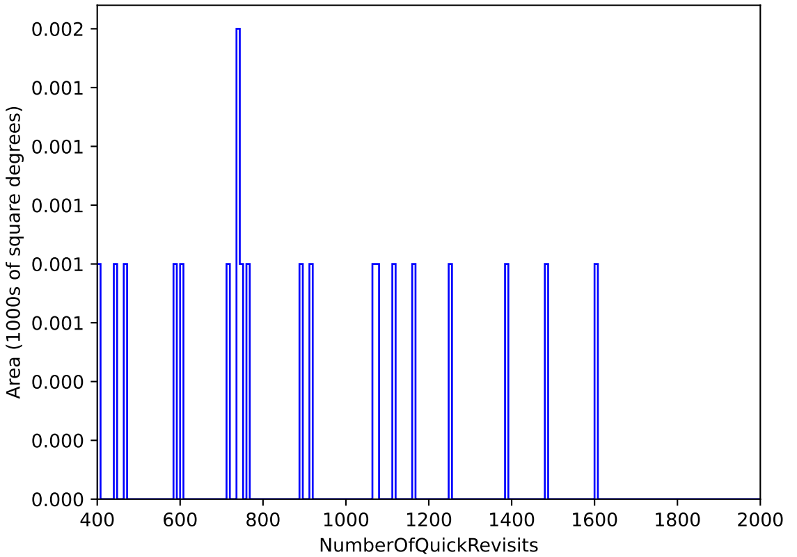
too_elab_r16_d2_ugrizy_v3.4_10yrs WFD: NumberOfQuickRevisits
