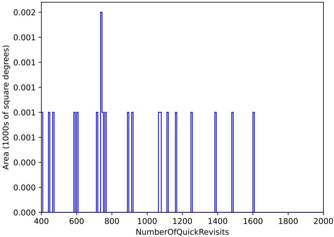
too_elab_r16_d2_ugrizy_v3.4_10yrs All sky: NumberOfQuickRevisits
