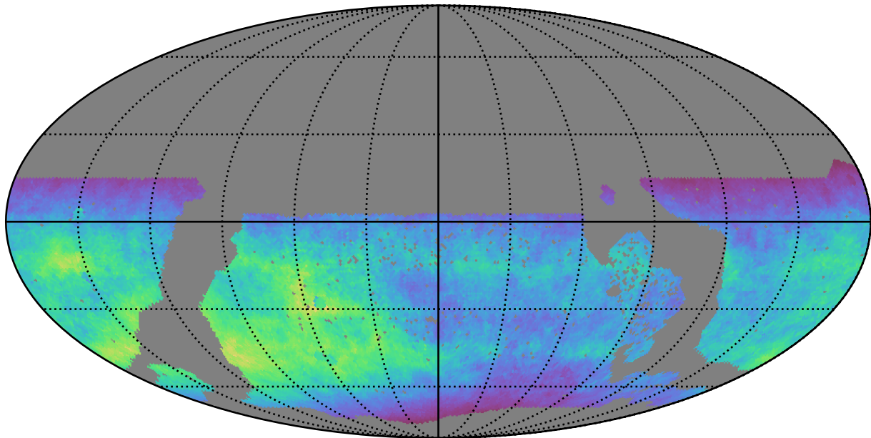
too_elab_r16_d2_ugrizy_v3.4_10yrs WFD z band: Normalized Teff
