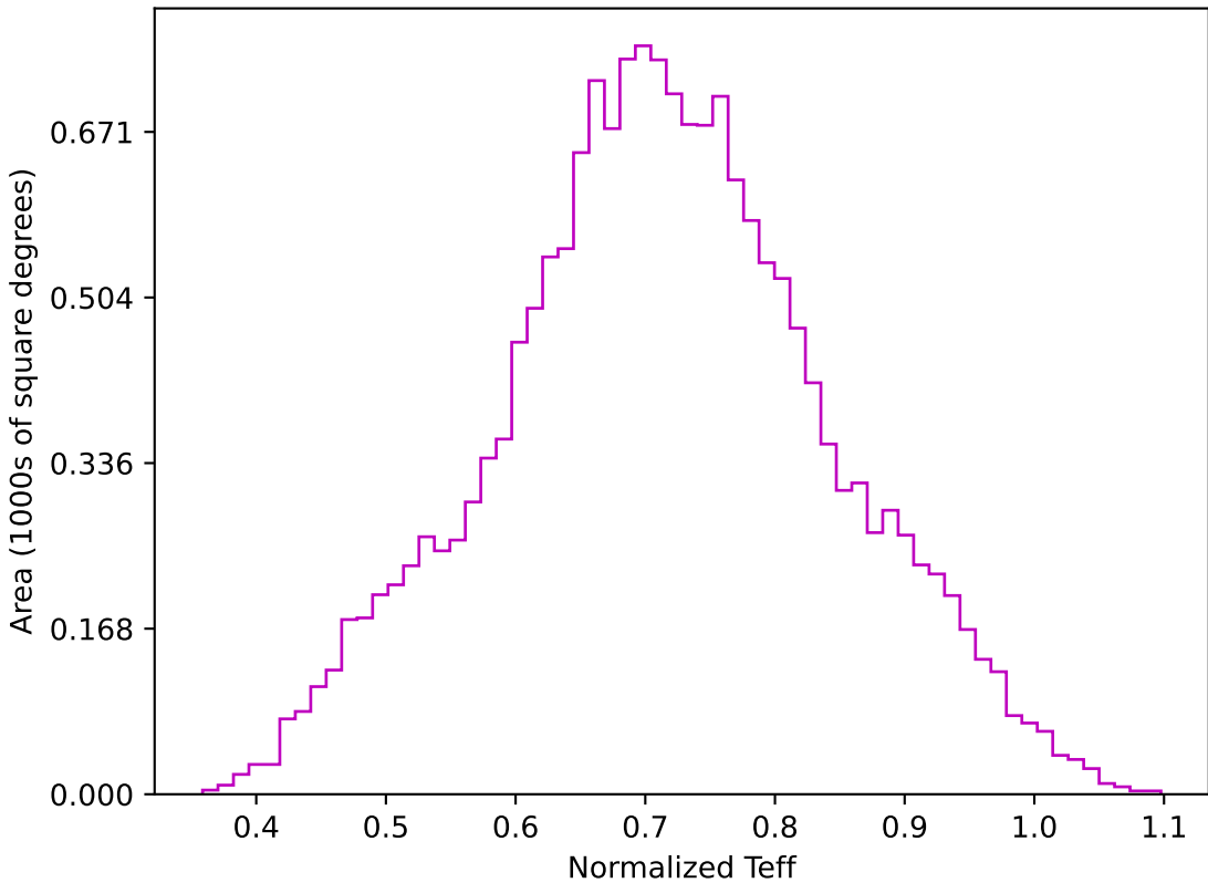
too_elab_r16_d2_ugrizy_v3.4_10yrs WFD z band: Normalized Teff
