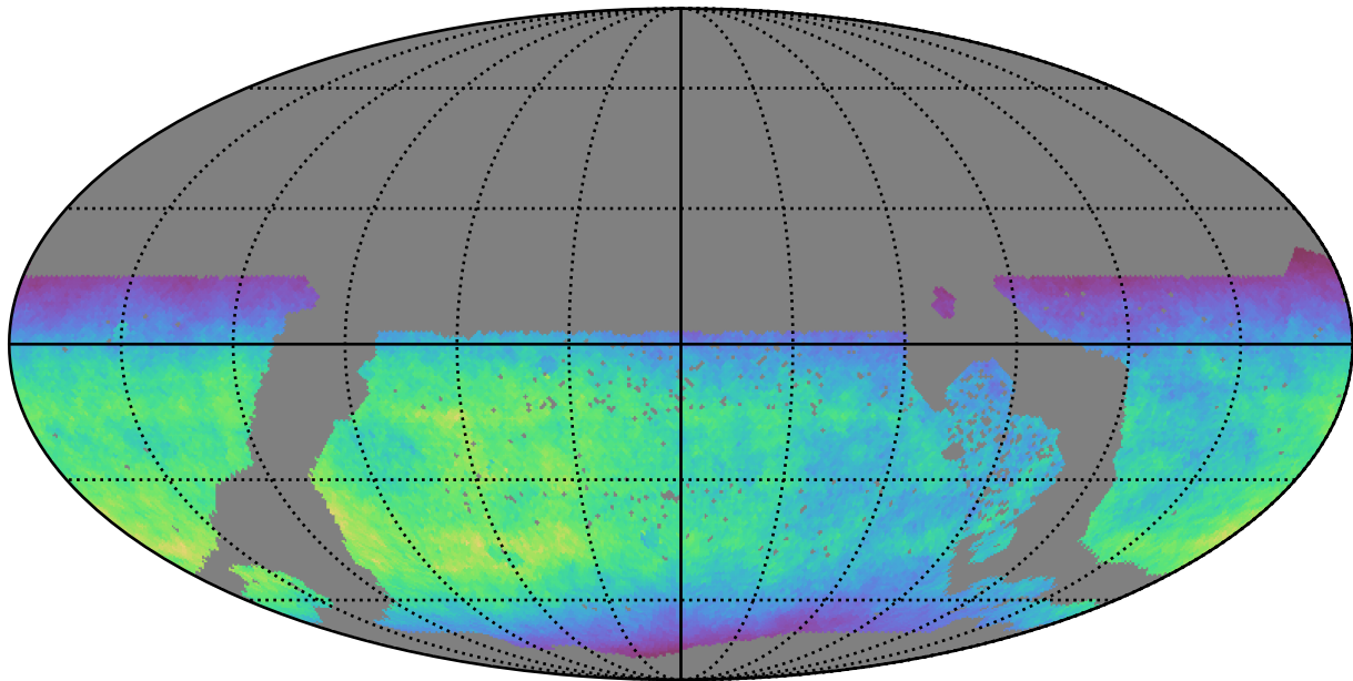
too_elab_r16_d2_ugrizy_v3.4_10yrs WFD y band: Normalized Teff
