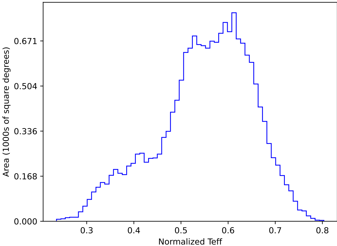
too_elab_r16_d2_ugrizy_v3.4_10yrs WFD y band: Normalized Teff
