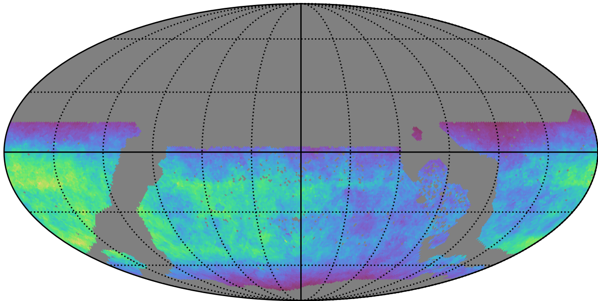
too_elab_r16_d2_ugrizy_v3.4_10yrs WFD u band: Normalized Teff
