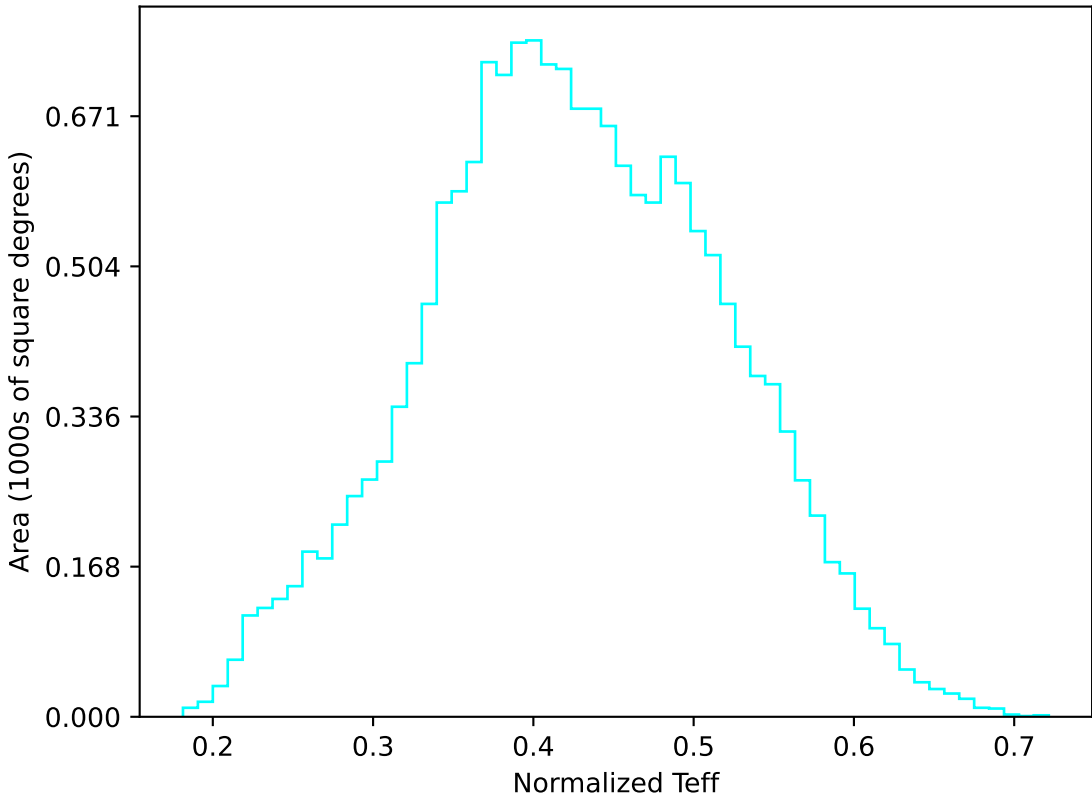
too_elab_r16_d2_ugrizy_v3.4_10yrs WFD u band: Normalized Teff
