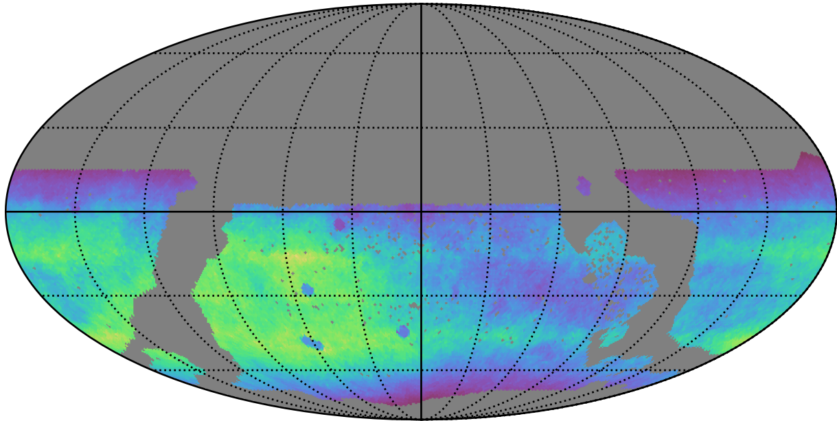
too_elab_r16_d2_ugrizy_v3.4_10yrs WFD r band: Normalized Teff
