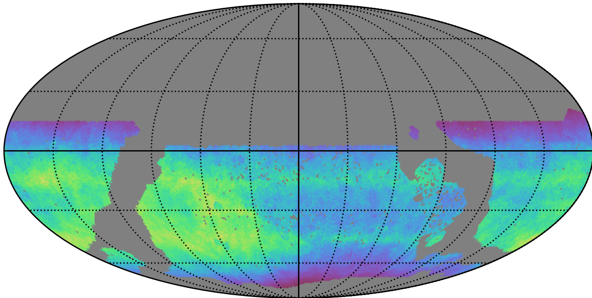
too_elab_r16_d2_ugrizy_v3.4_10yrs WFD i band: Normalized Teff
