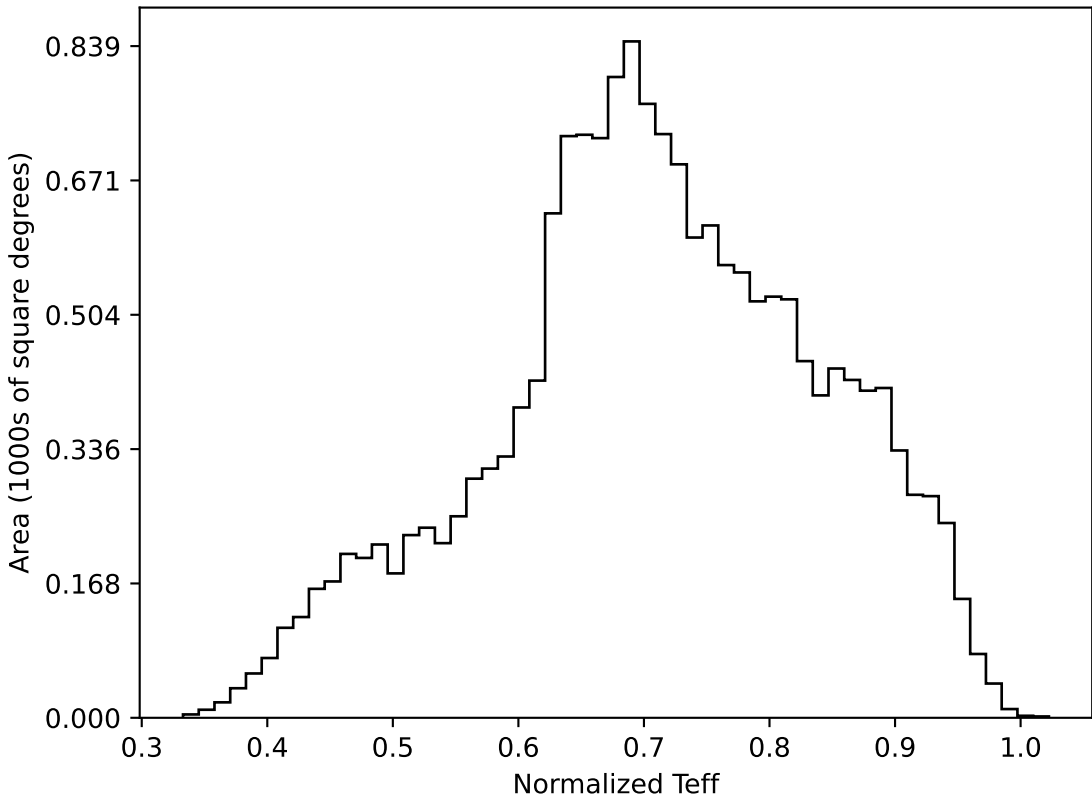
too_elab_r16_d2_ugrizy_v3.4_10yrs WFD all bands: Normalized Teff
