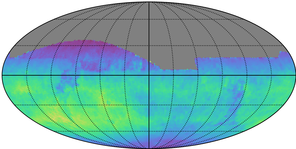
too_elab_r16_d2_ugrizy_v3.4_10yrs All sky z band: Normalized Teff
