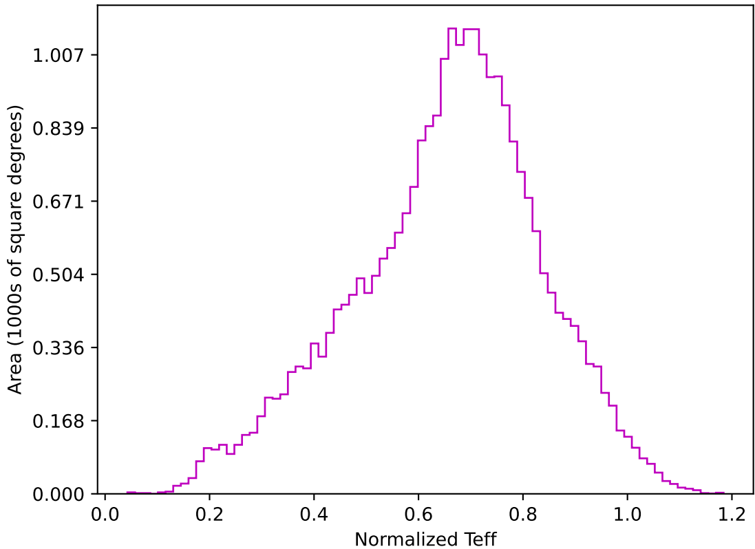
too_elab_r16_d2_ugrizy_v3.4_10yrs All sky z band: Normalized Teff
