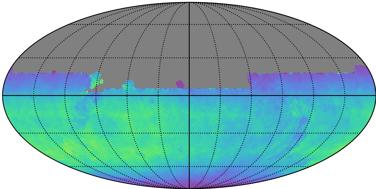
too_elab_r16_d2_ugrizy_v3.4_10yrs All sky y band: Normalized Teff
