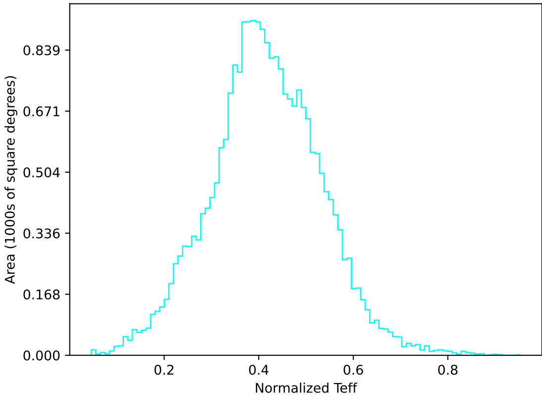
too_elab_r16_d2_ugrizy_v3.4_10yrs All sky u band: Normalized Teff
