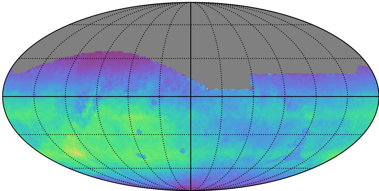
too_elab_r16_d2_ugrizy_v3.4_10yrs All sky r band: Normalized Teff
