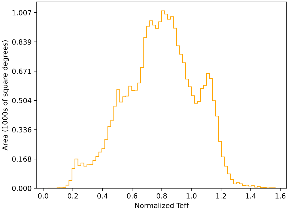
too_elab_r16_d2_ugrizy_v3.4_10yrs All sky r band: Normalized Teff
