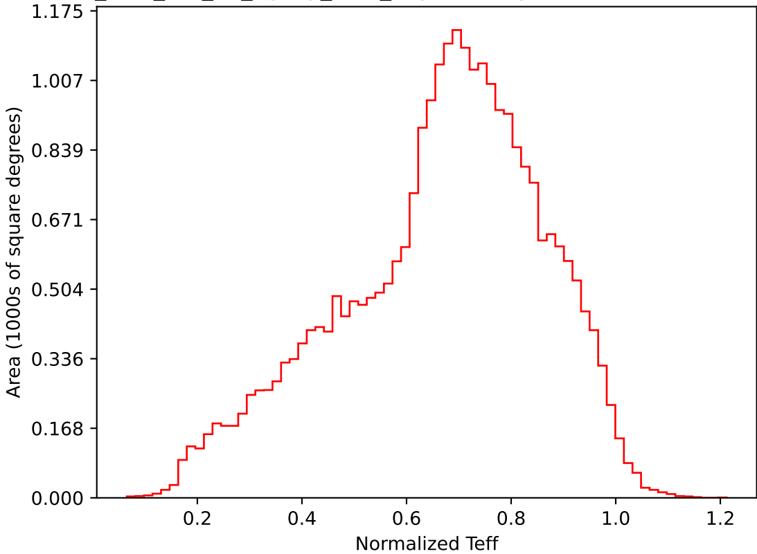
too_elab_r16_d2_ugrizy_v3.4_10yrs All sky i band: Normalized Teff
