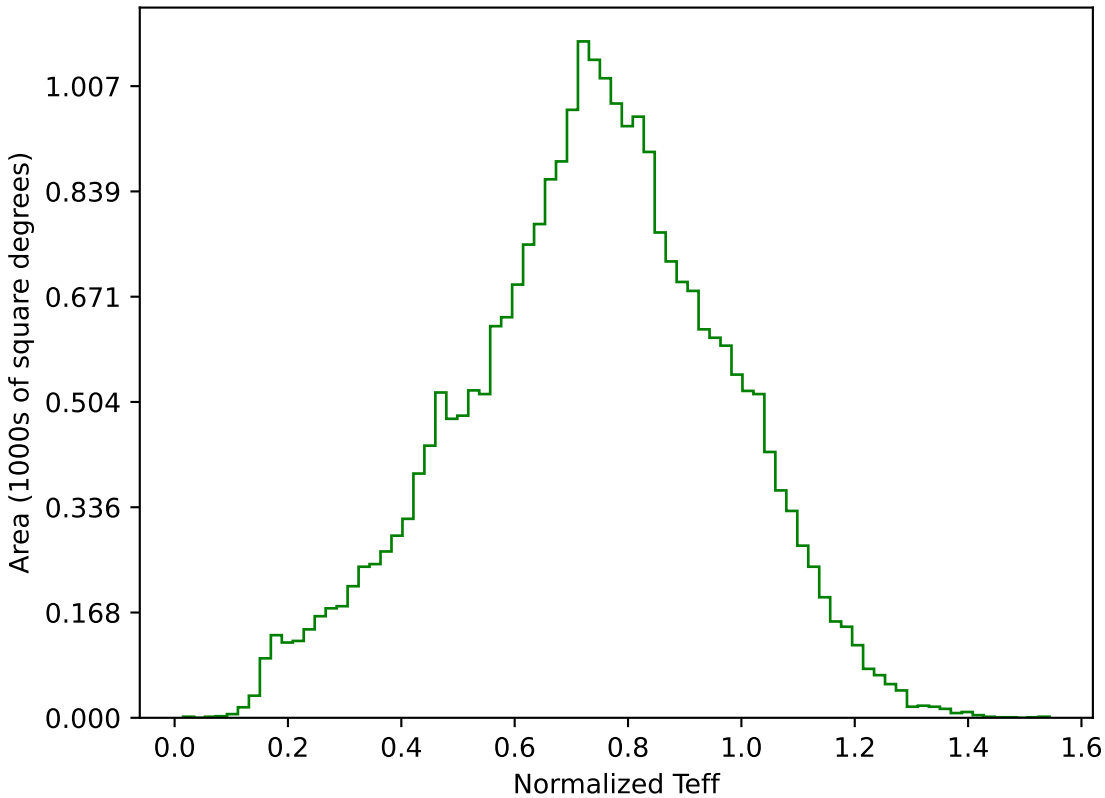
too_elab_r16_d2_ugrizy_v3.4_10yrs All sky g band: Normalized Teff
