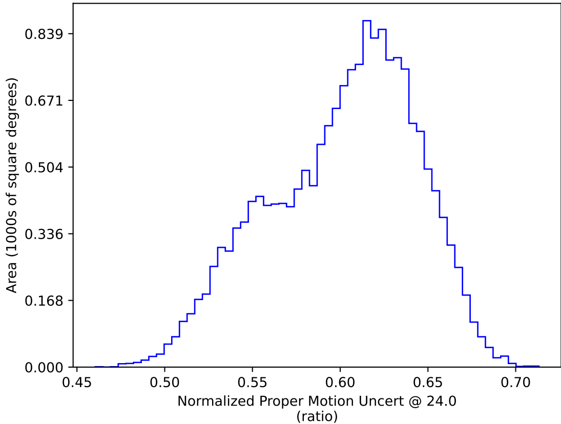
too_elab_r16_d2_ugrizy_v3.4_10yrs WFD: Normalized Proper Motion Uncert @ 24.0
