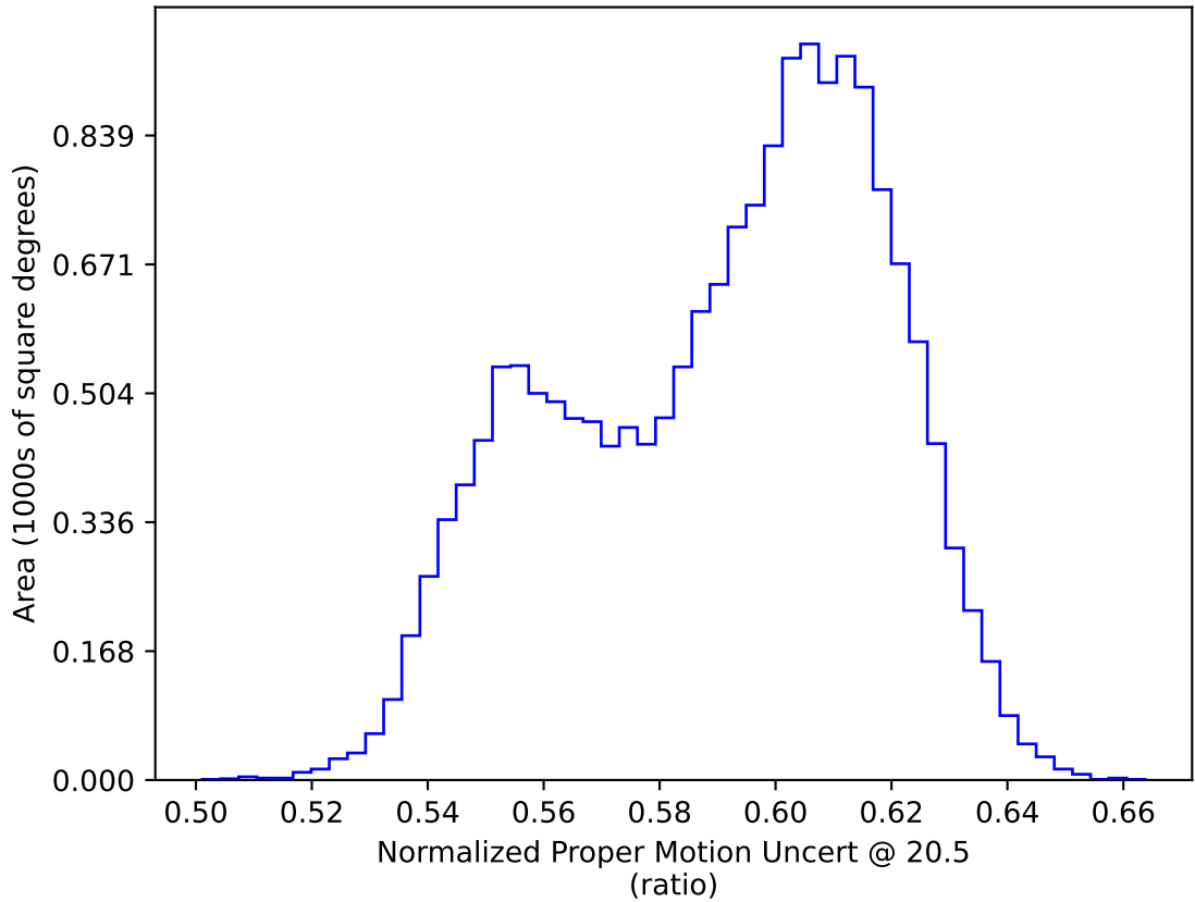
too_elab_r16_d2_ugrizy_v3.4_10yrs WFD: Normalized Proper Motion Uncert @ 20.5
