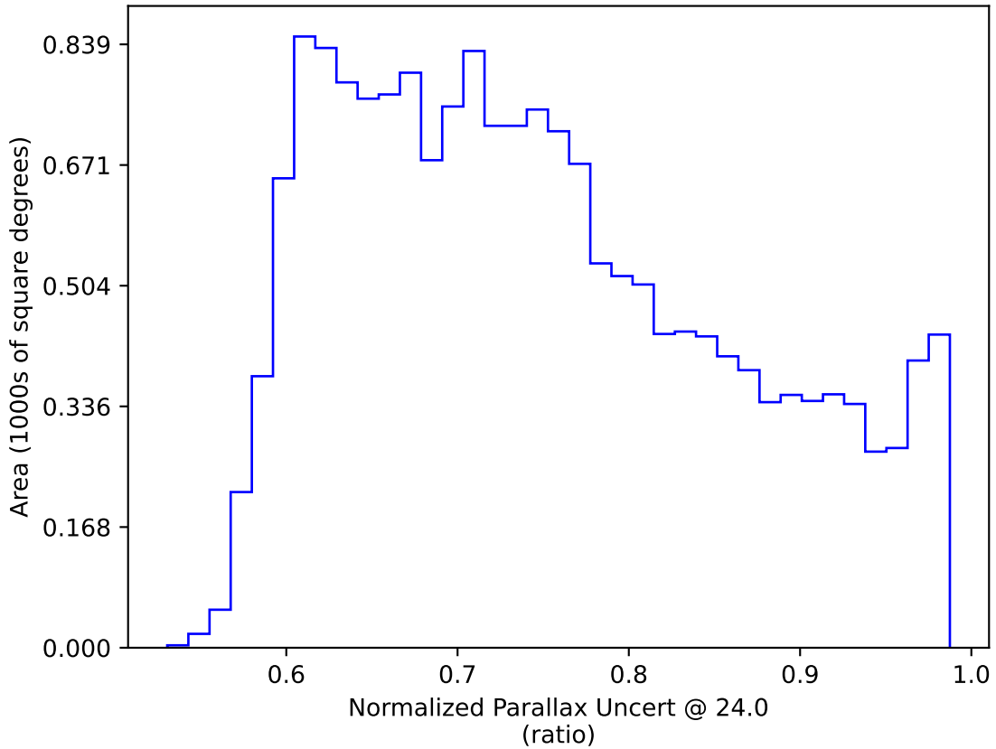
too_elab_r16_d2_ugrizy_v3.4_10yrs WFD: Normalized Parallax Uncert @ 24.0
