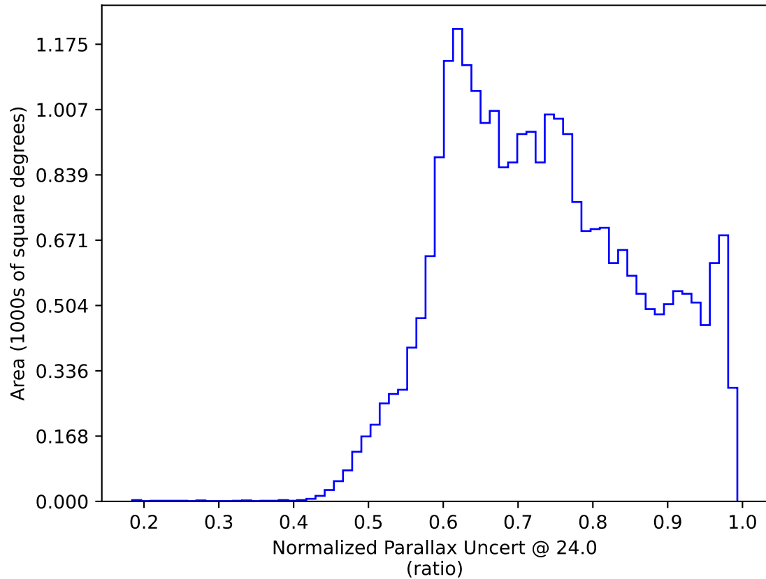
too_elab_r16_d2_ugrizy_v3.4_10yrs All sky: Normalized Parallax Uncert @ 24.0
