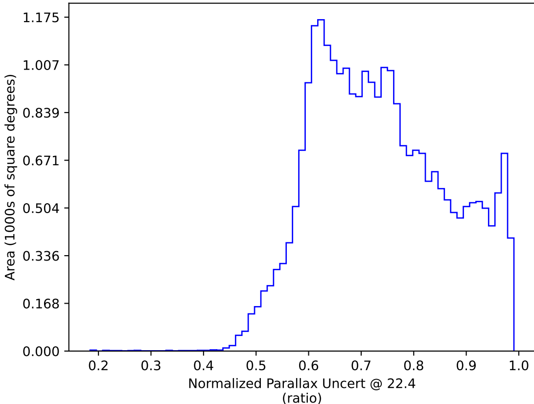
too_elab_r16_d2_ugrizy_v3.4_10yrs All sky: Normalized Parallax Uncert @ 22.4
