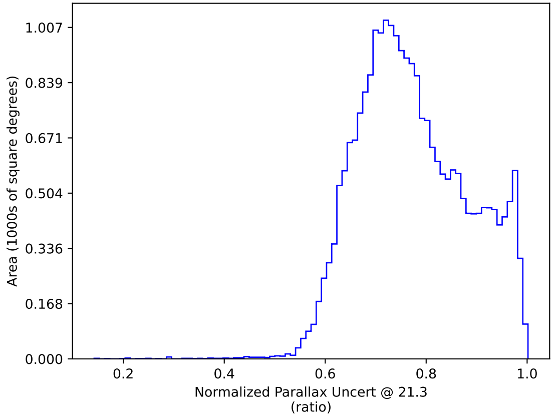
too_elab_r16_d2_ugrizy_v3.4_10yrs All sky y band only: Normalized Parallax Uncert @ 21.3
